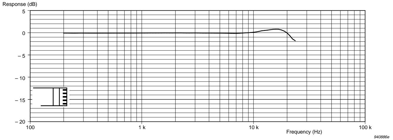
Fig.3.7 Typical free-field response (0° incidence) for the microphone with Protection Grid DB 3420
