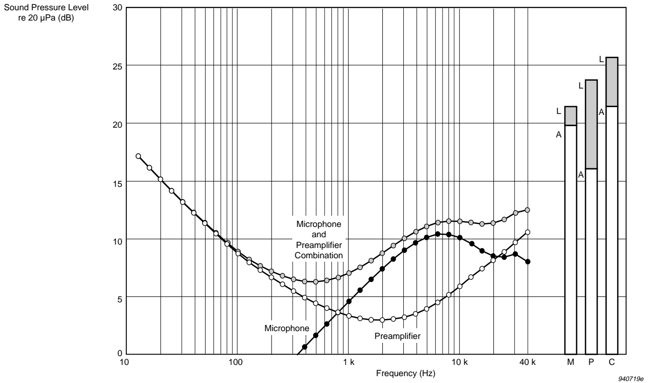
Fig. 5.16 1/3-octave-band inherent noise spectrum. The shaded bar graphs are the broadband (20 Hz to 40 kHz) noise levels and the white bar graphs the A-weighted noise levels of the microphone (M), 1/2" Microphone Preamplifier Type 2669 (P) and microphone and preamplifier combination (C)
