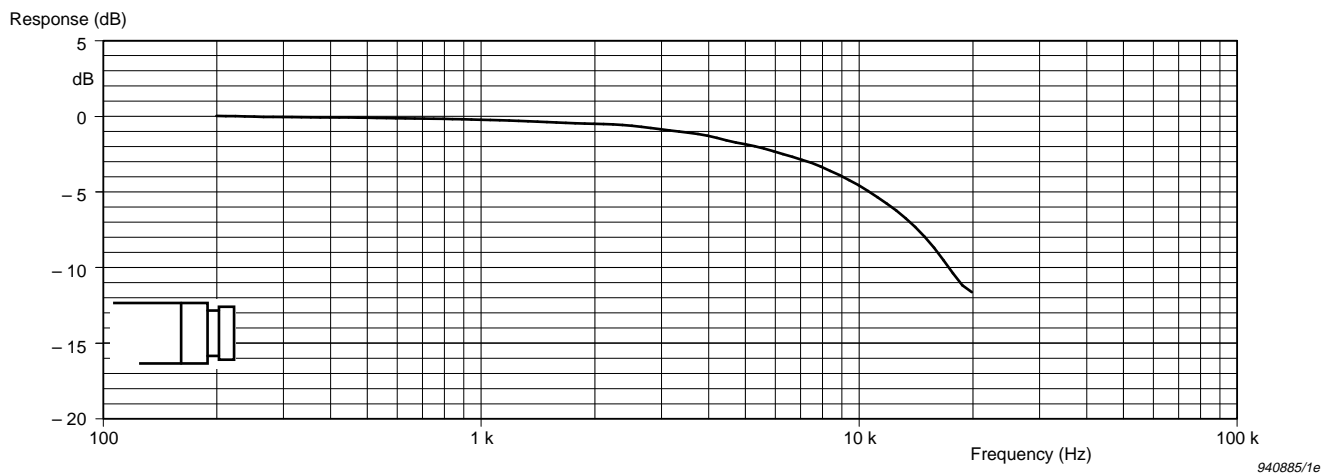
Fig. 2.13 Typical random-incidence response for the microphone without protection grid
