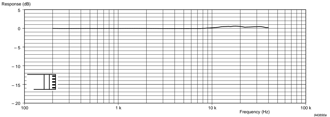
Fig 5.7 Typical free-field response ( 0^\circ incidence) for the microphone with Protection Grid DB 3421
