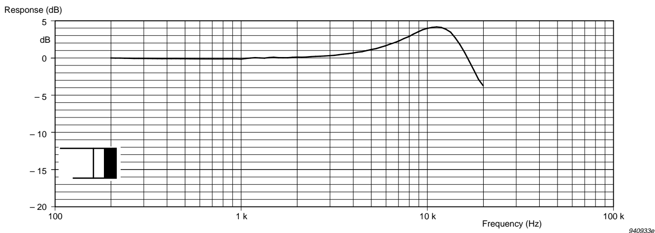
Fig.2.11 Typical free-field response ( 0^\circ -incidence) for the microphone with Random Incidence Corrector DZ 9566
