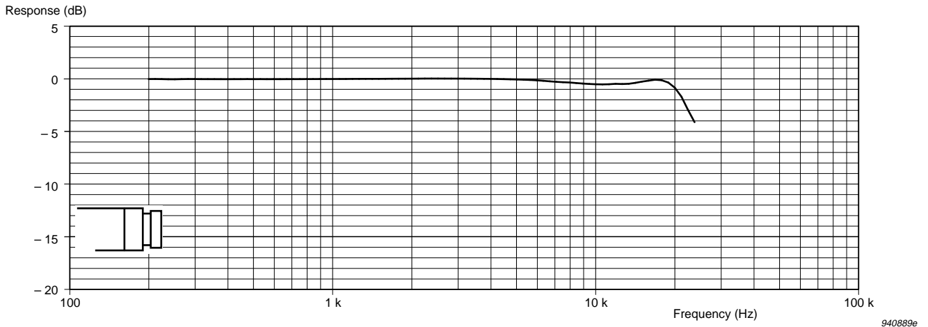
Fig 4.9 Typical free-field response ( 0^\circ incidence) for the microphone without protection grid
