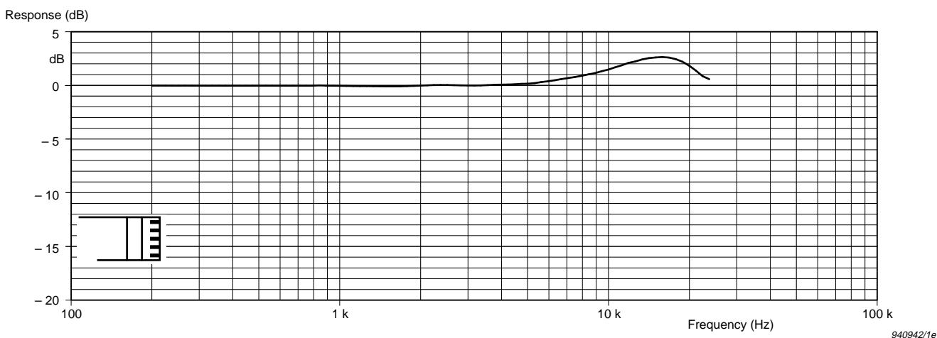
Fig. 6.10 Typical random-incidence response for the microphone with Protection Grid DB 3421
